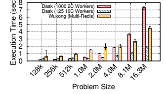
Figure 12: SVC.
