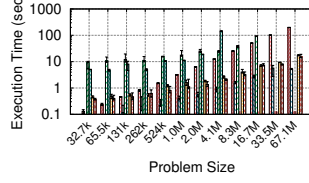
Figure 14: TSQR (log-scale).
