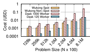
Figure 18: SVD1 cost.
