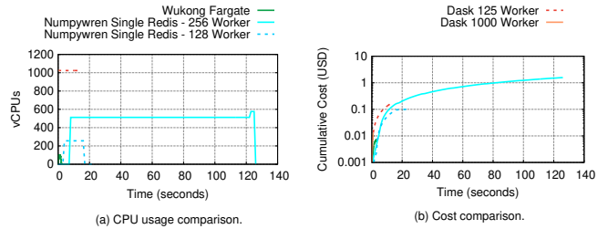
Figure 20: TSQR CPU usage and cost timeline.
