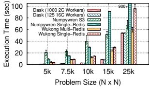
Figure 13: GEMM.
